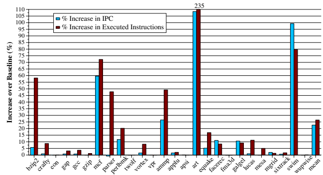
Figure 2. Increase in IPC and executed instructions due to runahead execution.
